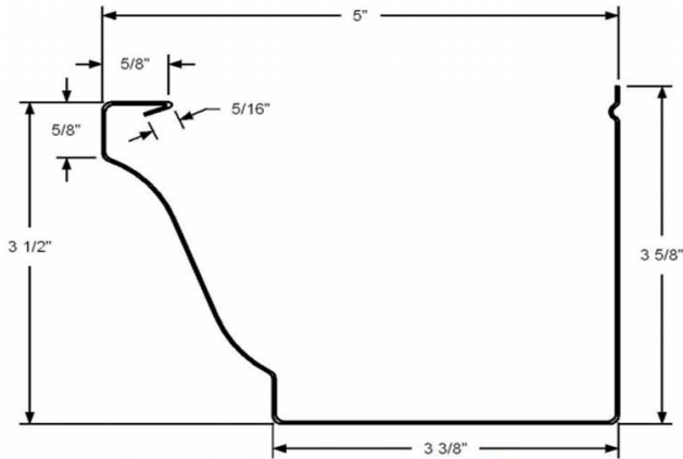
5" and 6" Ogee - No Wing
