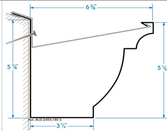
Eclipse Millennium Gutter
