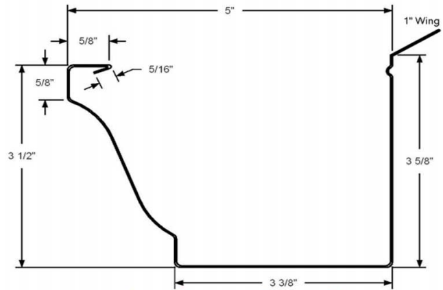
5" and 6" Ogee - With Wing
